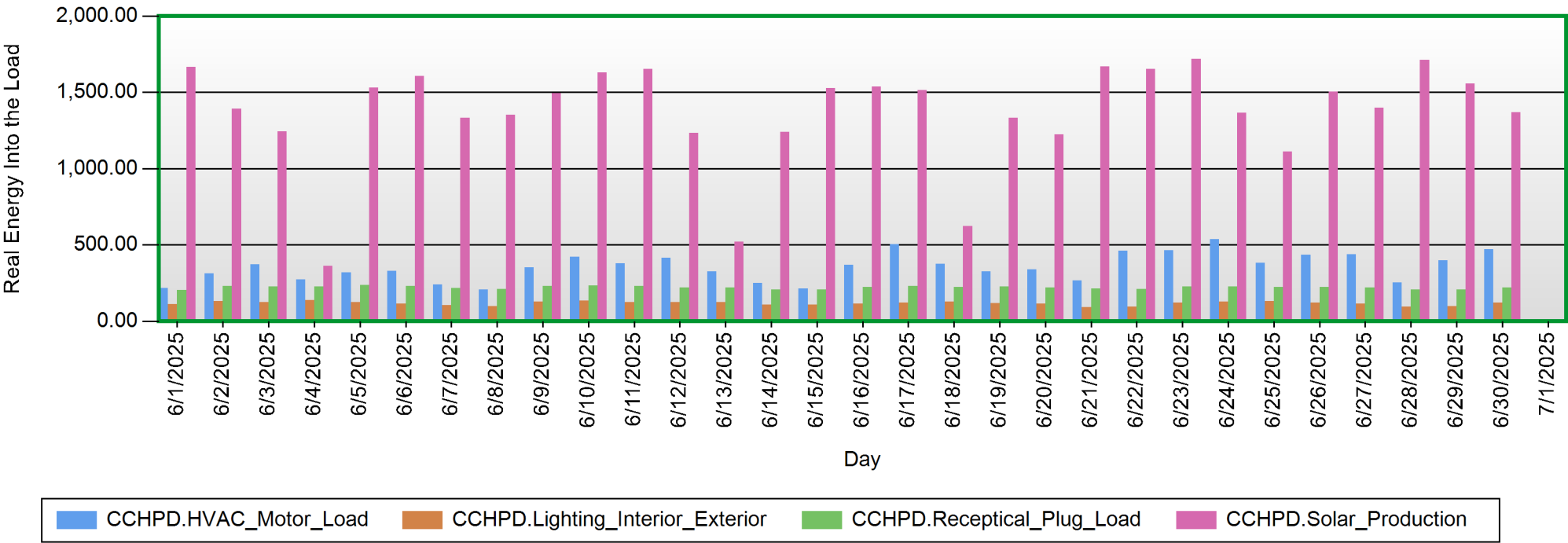
Energy Usage 00:00 - 00:00
