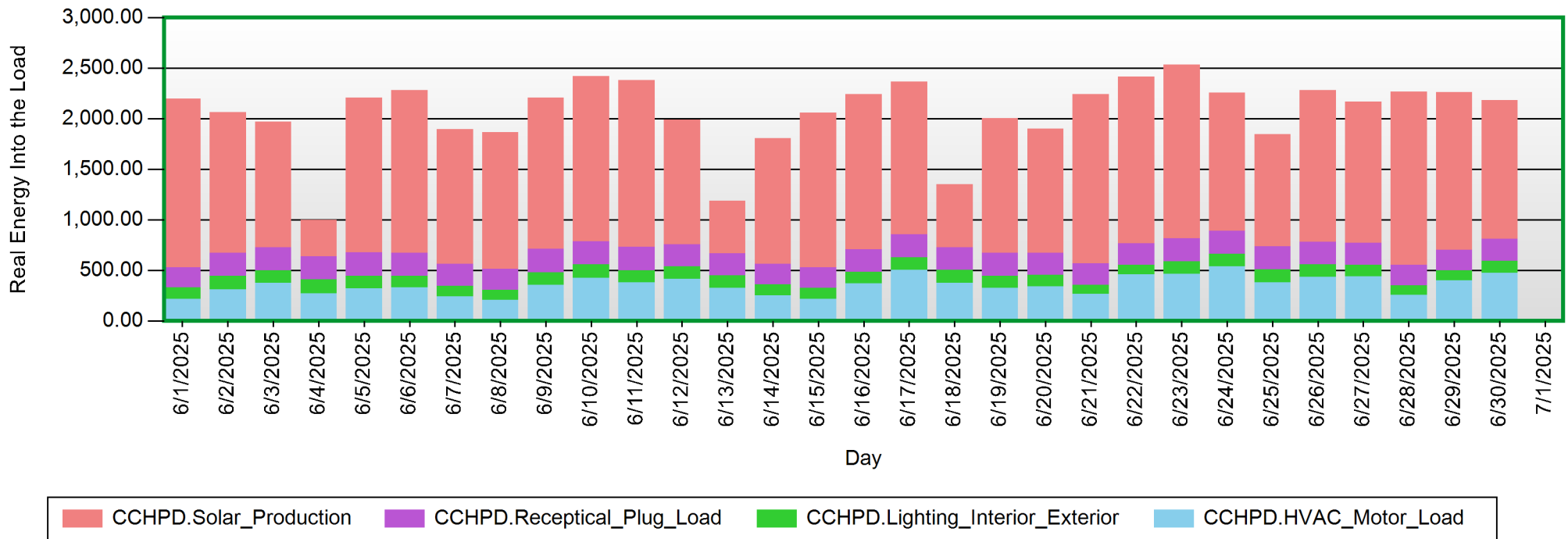
Energy Usage 00:00 - 00:00
